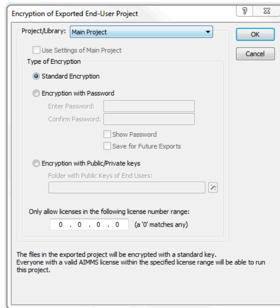
Figure 5.2: Encryption of Exported End-User Project
